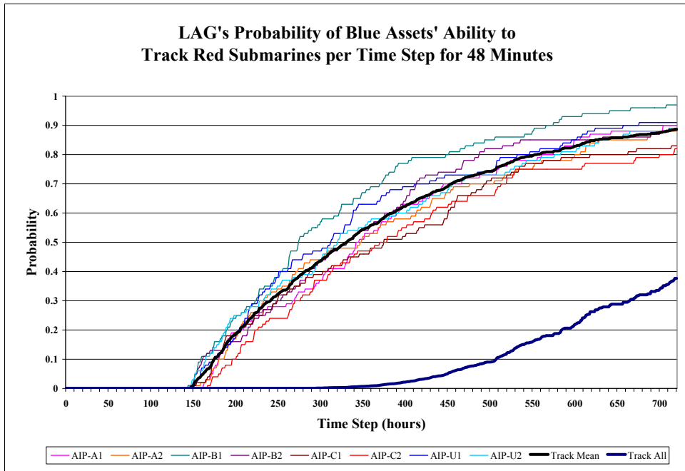
Figure 166: Probability that Blue Assets can Successfully Track Red Submarines per Time Step in 48 Minutes for LAG Alternative
