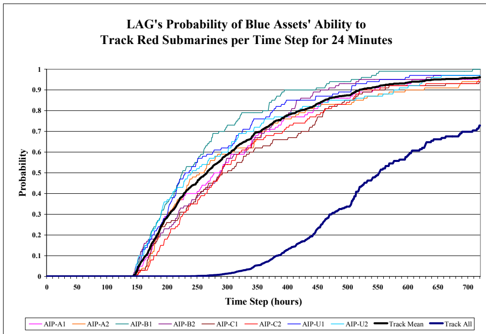
Figure 162: Probability that Blue Assets can Successfully Track Red Submarines per Time Step in 24 Minutes for LAG Alternative
