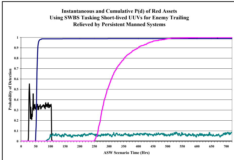
Figure 121: The Instantaneous and Cumulative Probability of Detection of an Enemy Submarine Leaving Port
