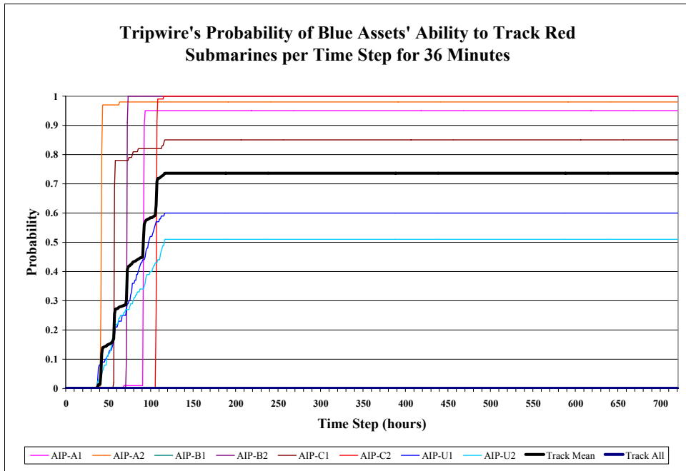
Figure 137: Probability that Blue Assets can Successfully Track Red Submarines per Time Step in 36 Minutes for Tripwire Alternative
