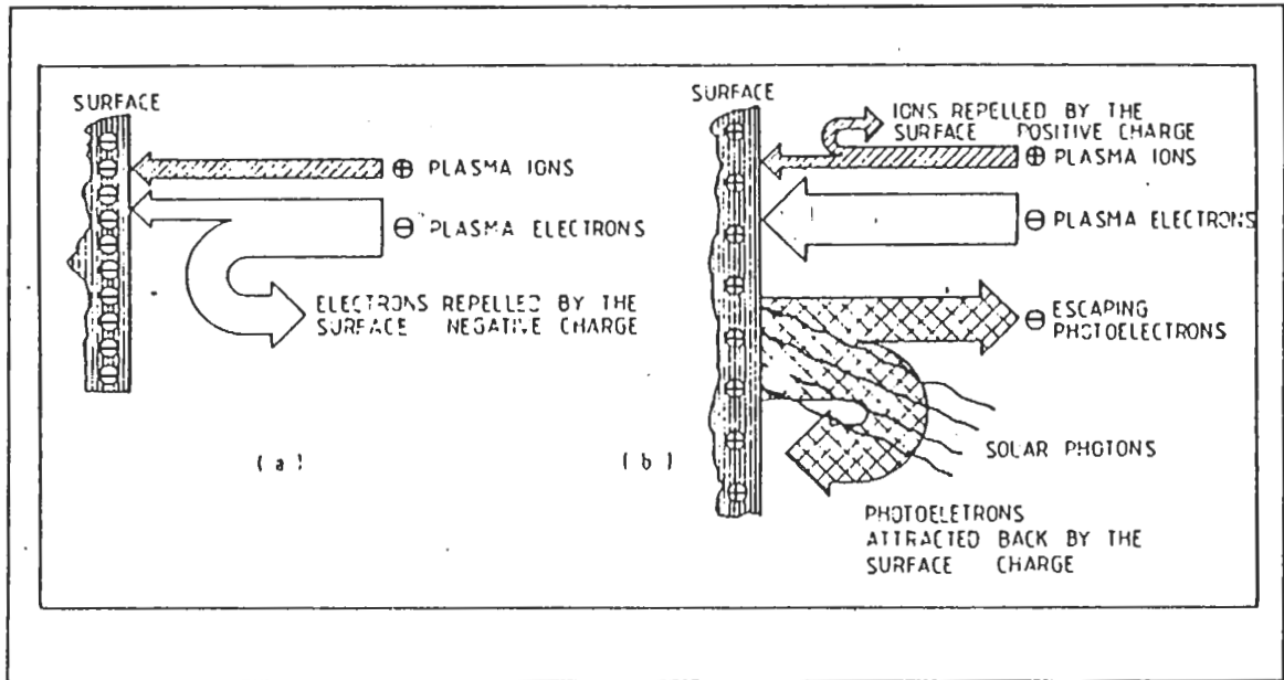
Figure 1. Qualitative illustration of the charging: of a surface by a plasma. (a) Surface in shadow (b) Surface in sunlight [Ref.1]
