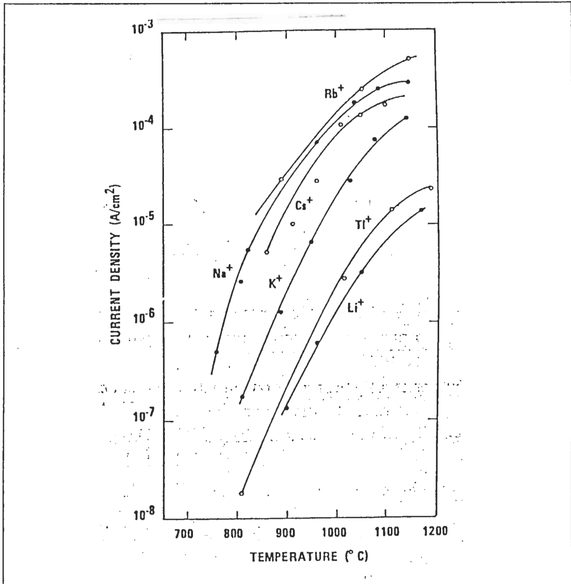
Figure 14. Typical current densities obtainable for the various emitters: as a function of temperature. [Ref.13]
