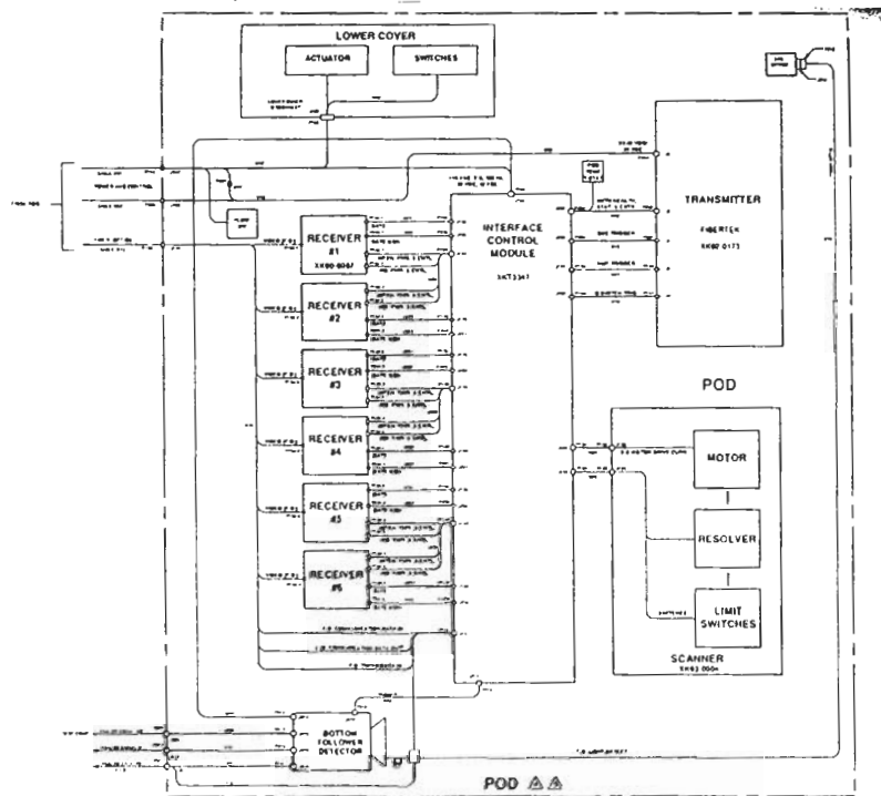
Figure 32: ML(A) sensor block diagram. (Kaman, 1993)
