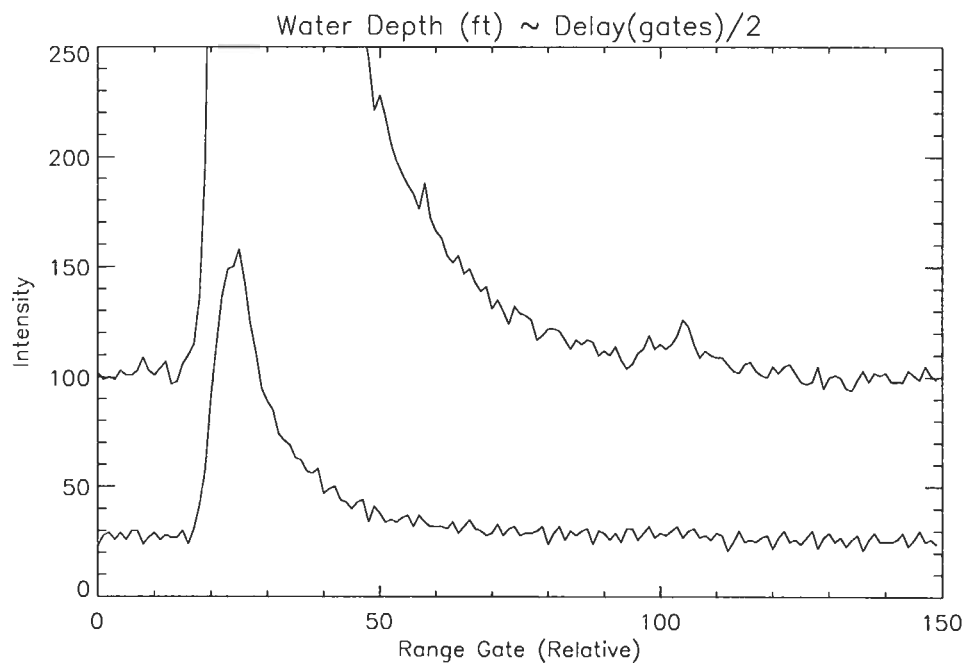
Figure 35: Line plot of row 564, OWL data set D0534.
