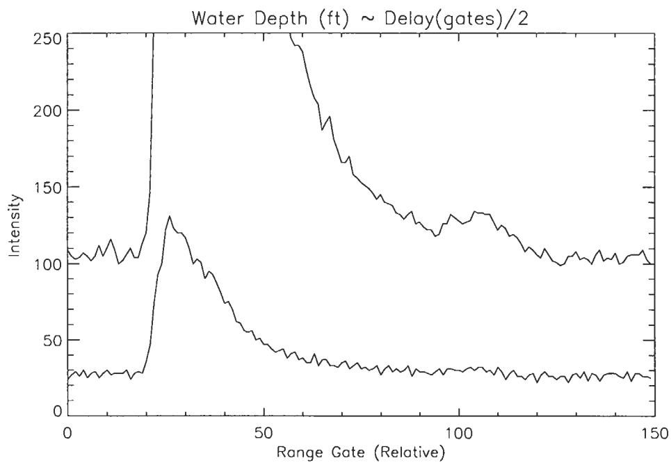
Figure 37: Line plot of row 1656, OWL data set D0534.
