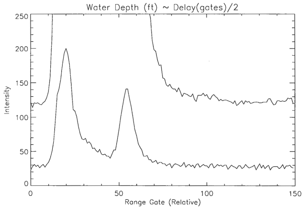
Figure 48: Line plot of row 5342, OWL data set D0534.
