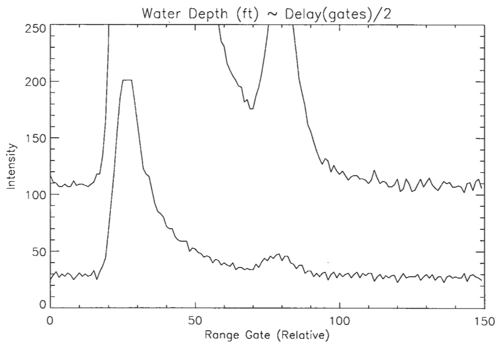
Figure 43: Line plot of row 4257, OWL data set D0534.
