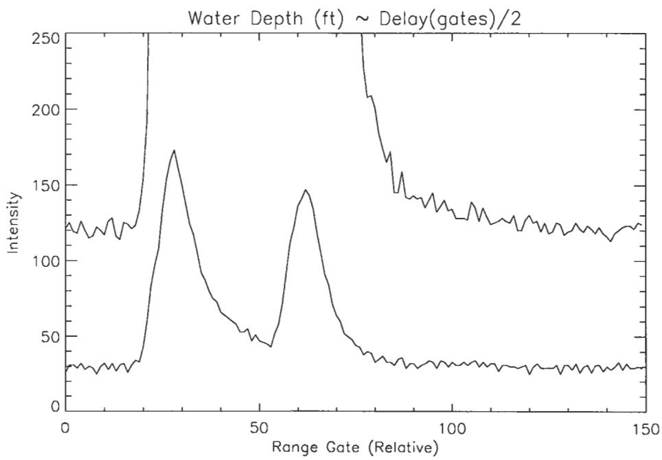
Figure 46: Line plot of row 4940, OWL data set D0534.
