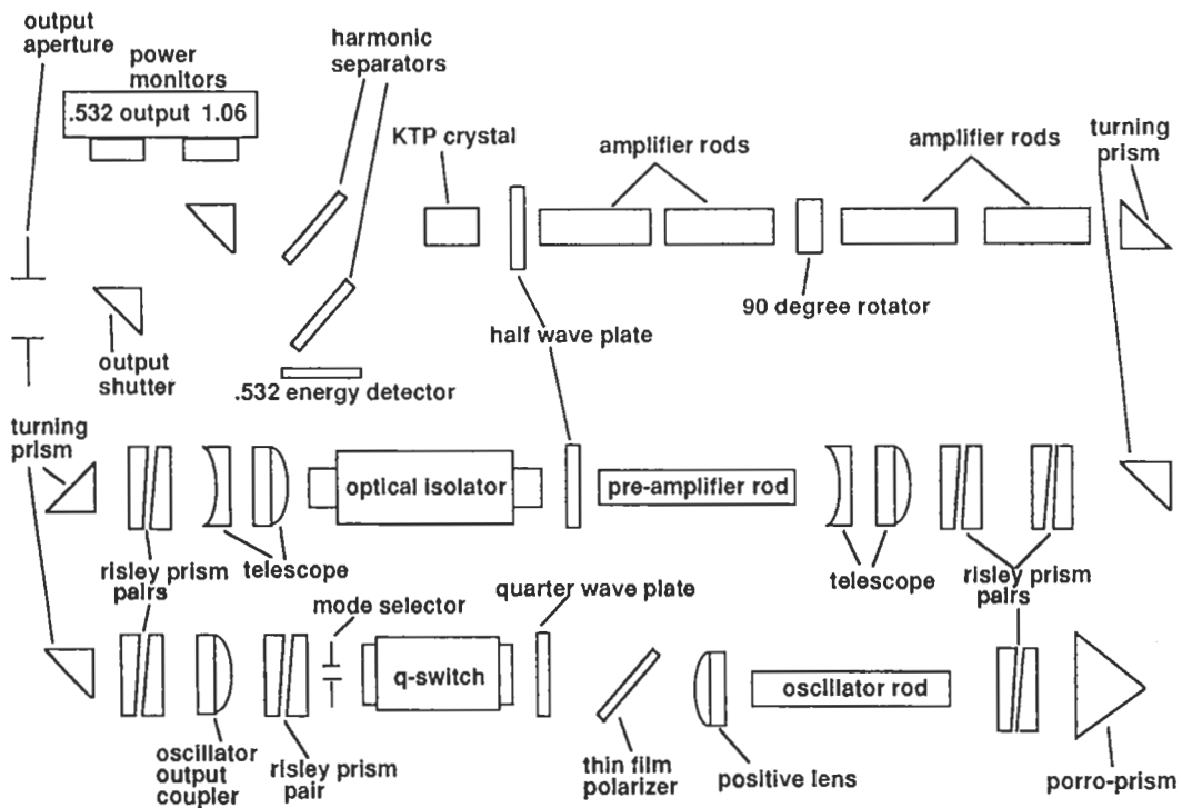
Figure 28: ML(A) Nd:YAG laser schematic. (Kaman, 1993)
