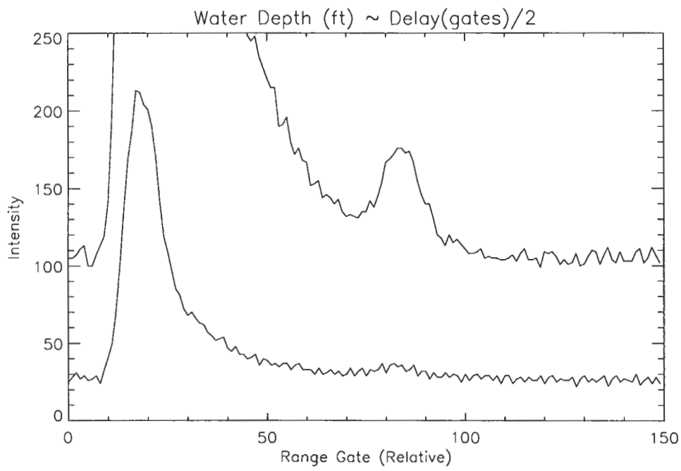
Figure 41: Line plot of row 3720, OWL data set D0534.
