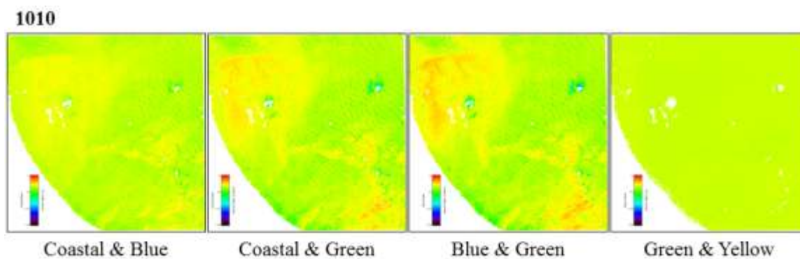
Figure 27. Derived depths for each band combination for Image 1010 (most forward-looking)
