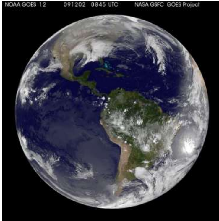
Figure 11. An example of sun glint on the ocean's surface (image captured by the Geostationary Operational Environmental Satellite (GOES) on 2 December 2009) (From http://rsd.gsfc.nasa.gov/goes/text/hotstuff.html )
