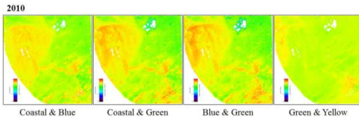
Figure 28. Derived depths for each band combination for Image 2010
