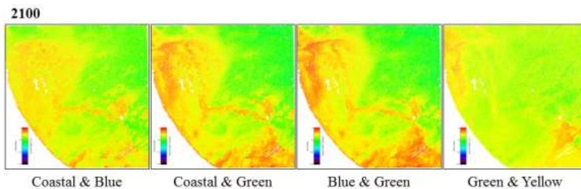
Figure 29. Derived depths for each band combination for Image 2100 (most nadir)
