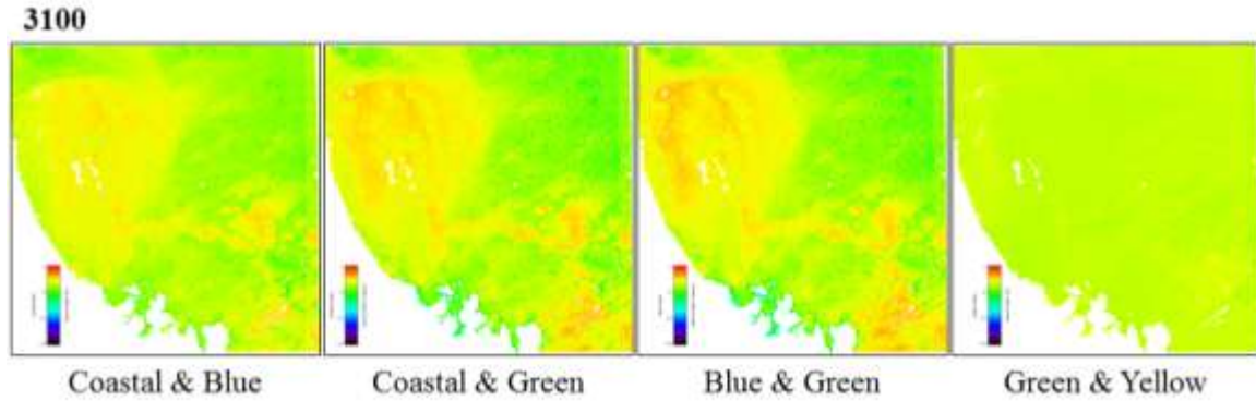
Figure 30. Derived depths for each band combination for Image 3100
