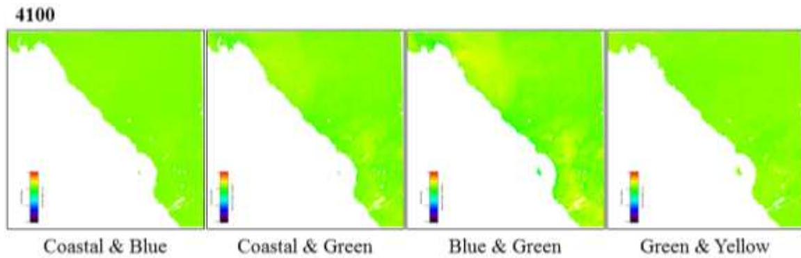
Figure 31. Derived depths for each band combination for Image 4100 (most backward-looking)
