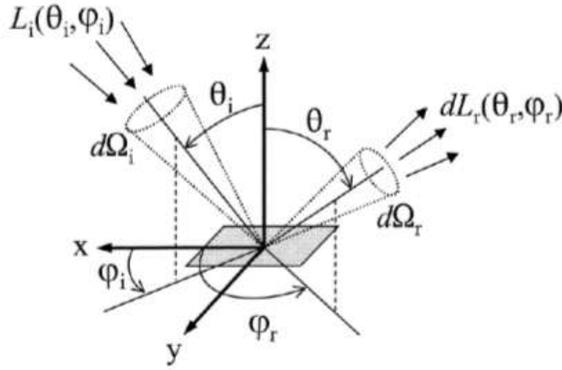
Figure 7. Reflection geometry used in the definition of BRDF (From McConnon [2010])
