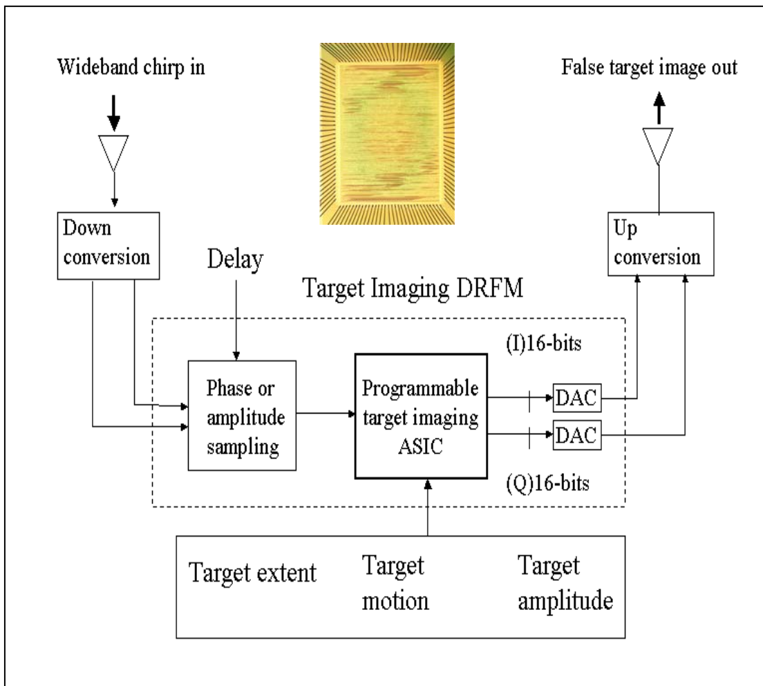
Figure 4: Block diagram of the false target image synthesizer.
