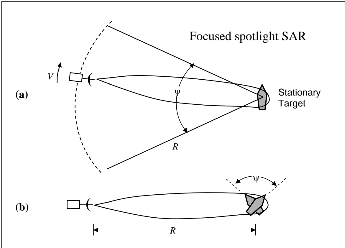
Figure 2: (a) Focused spotlight synthetic aperture radar (SSAR) mode and (b) Inverse synthetic aperture radar (ISAR) mode.
