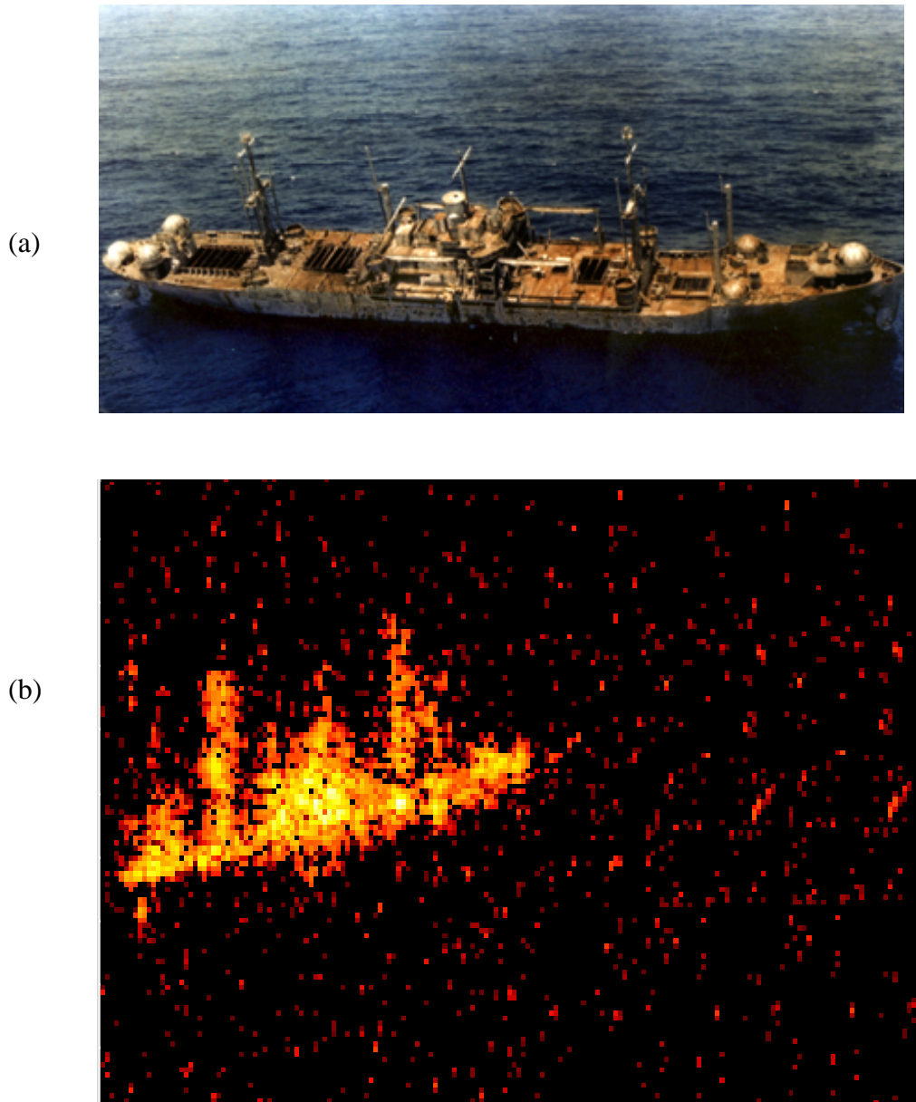
Figure 3: (a) the USS Crockett and (b) an AN/APS-137 ISAR image of the USS Crockett [3].
