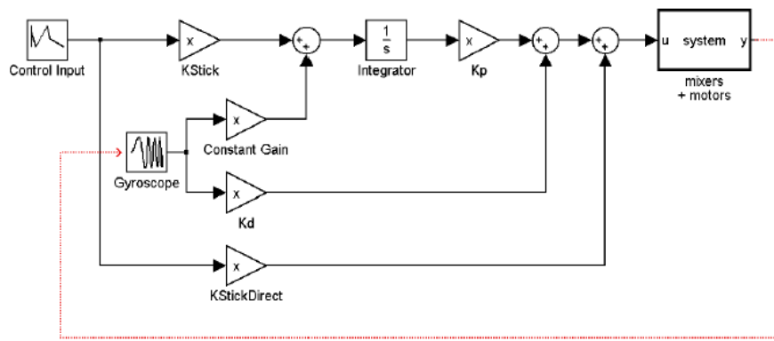
Figure 9. Heading Hold algorithm (From [8])
