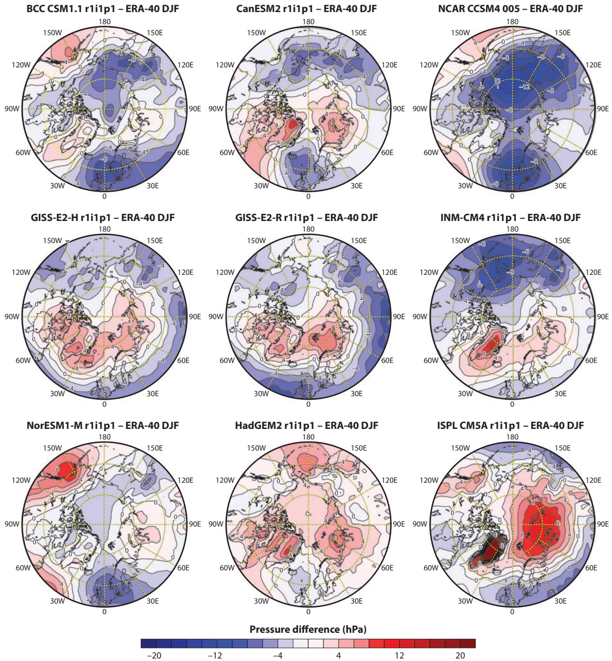
Figure 6 Differences in winter mean sea-level pressure averaged from 1979 to 2002 for nine CMIP5 global climate models versus ERA-40 (European Center for Medium-Range Weather Forecasts 40-year reanalysis data).
