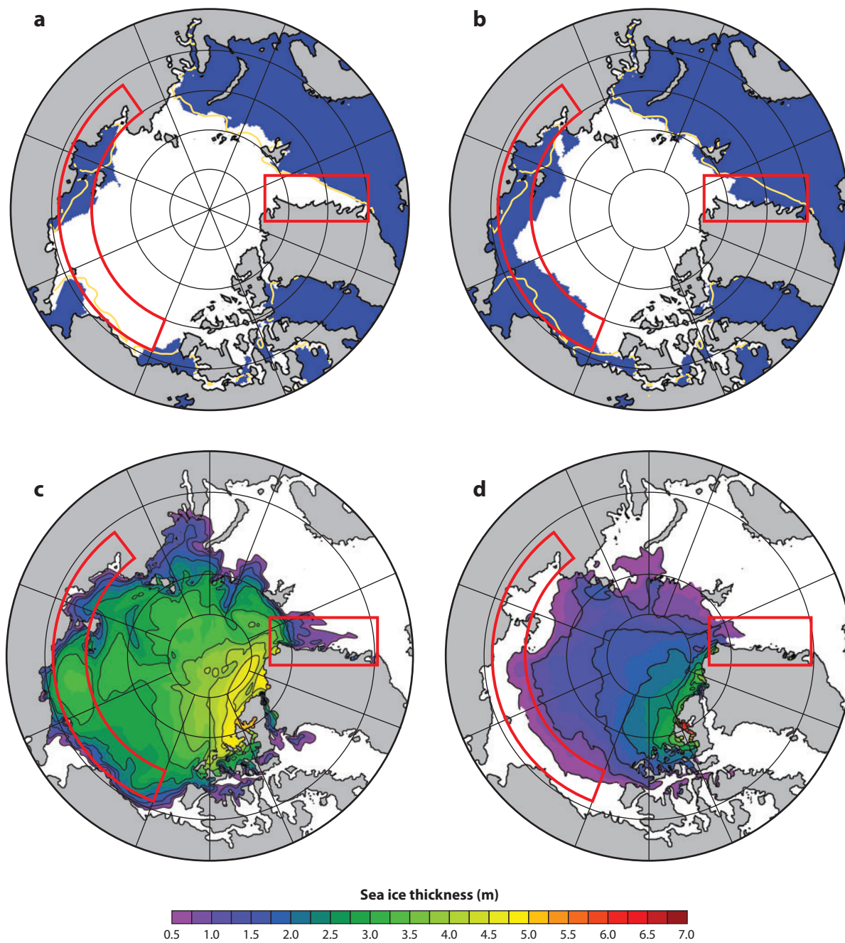
Figure 3 Comparison of (a,b) observed (NSIDC) September ice extent with (c,d) NAME modeled ice extent and thickness during (a,c) 1988 and (b,d) 2002.
