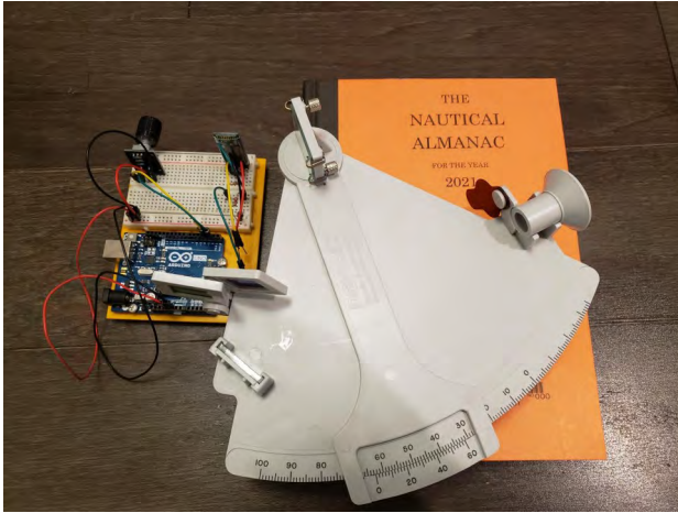
Mark 3 Sextant, Arduino Uno with breadboard. Photo Credit: Eric Peterson
